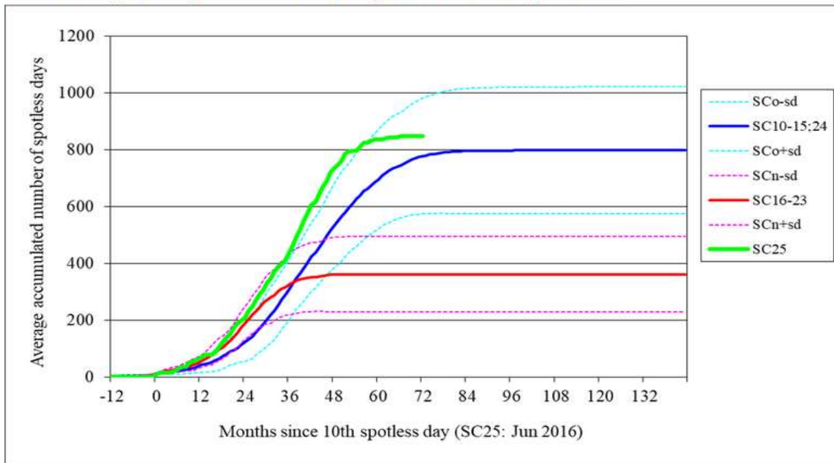
Evolution of spotless days in SC24-25 and comparison with other cycle transits
