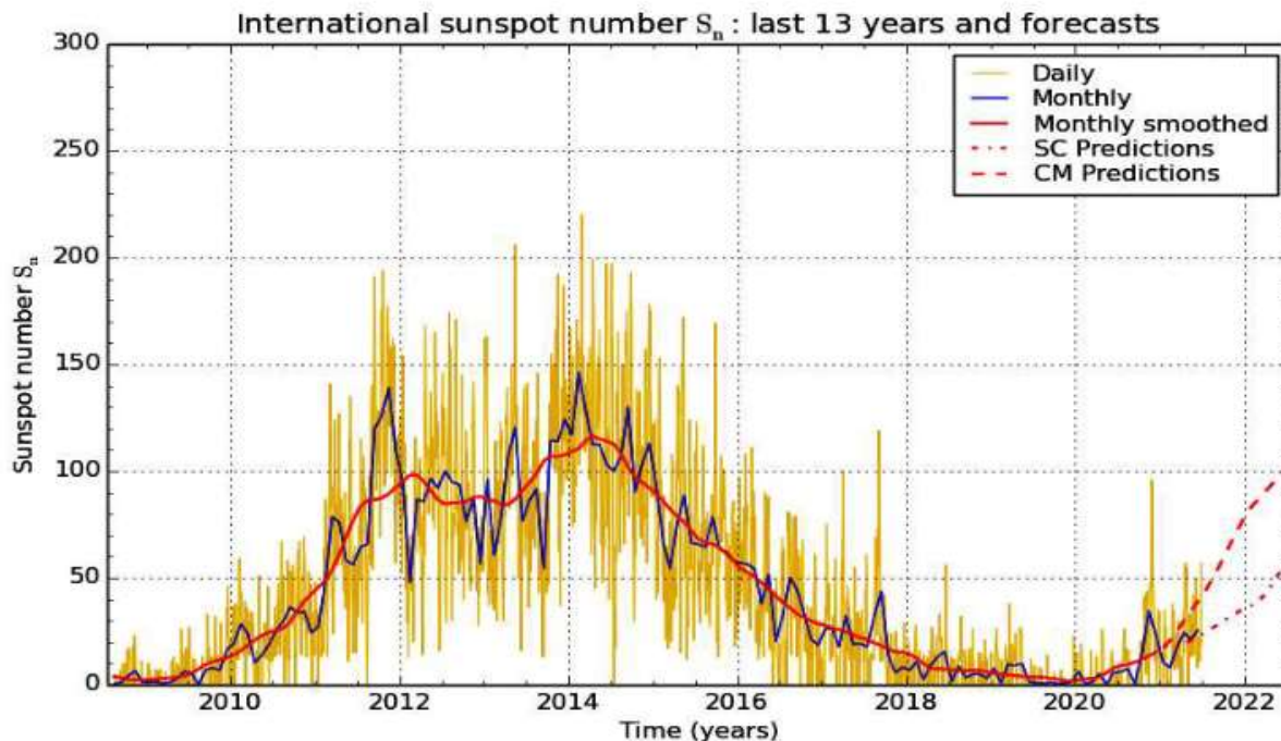
SILSO graphics ( http://sidc.be/silso ) Royal Observatory of Belgium 2021 July 2
