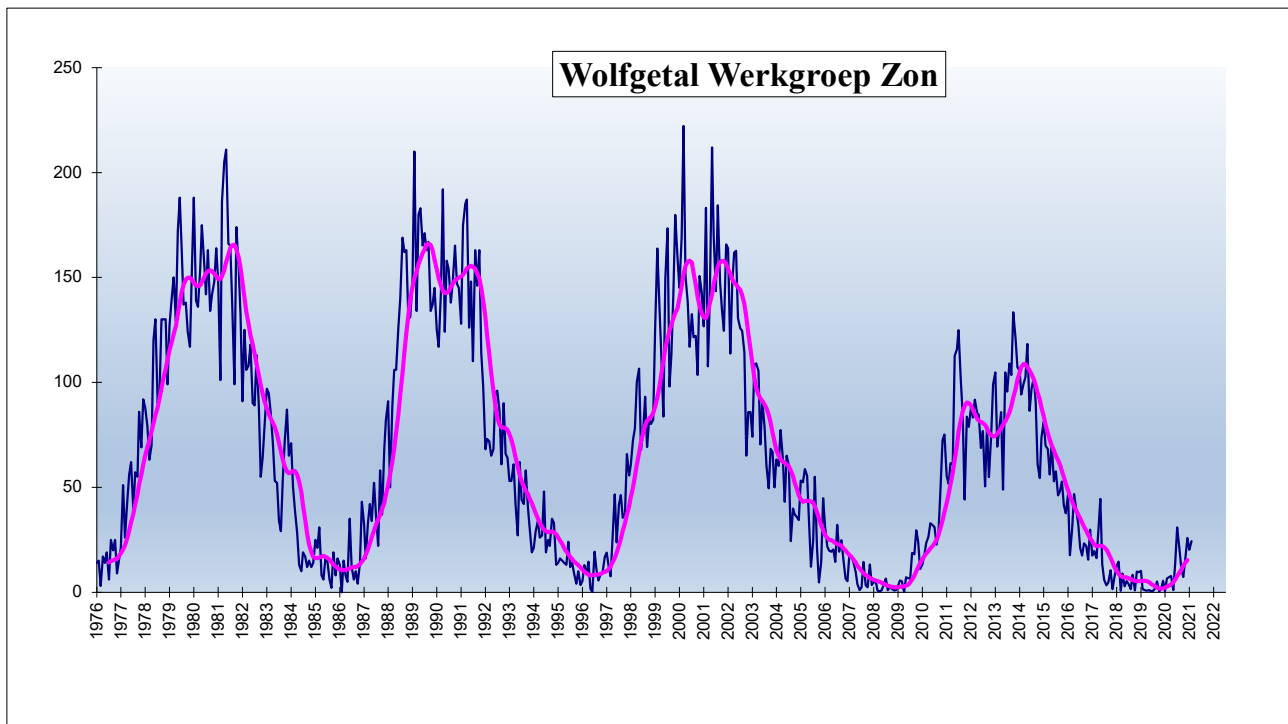
SILSO graphics ( http://sidc.be/silso ) Royal Observatory of Belgium 2021 July 2
