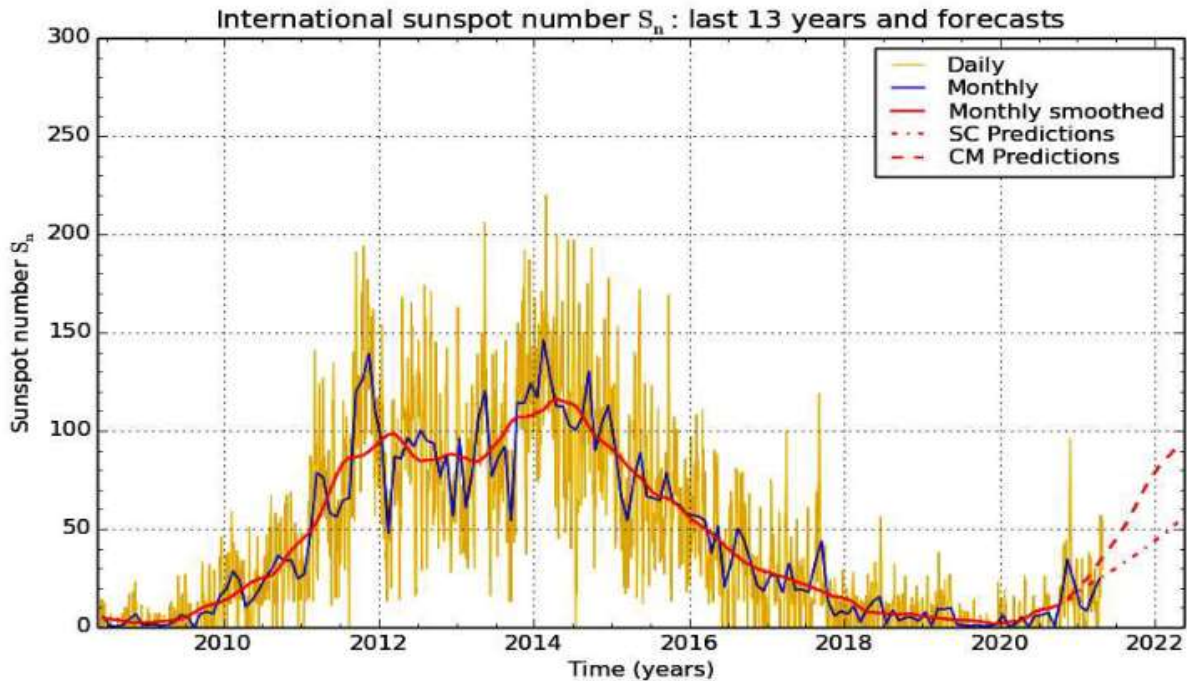
SILSO graphics ( http://sidc.be/silso ) Royal Observatory of Belgium 2021 May 1
