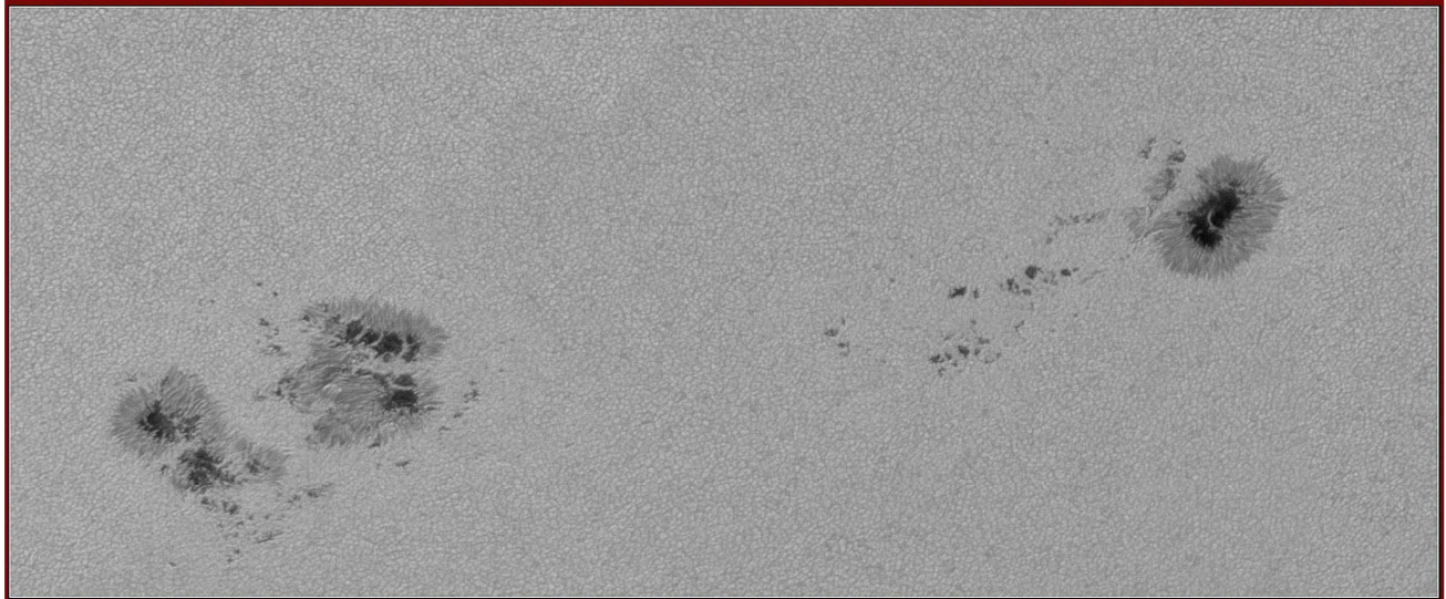
8 Sep 2021, ~12:24h UT, Sunspots, AR2866 & 2868. Takahashi TOA-150b, Baader Herschel wedge, Baader ND & Solar Continuum filters. Televue Powermate 2.5x, ZWO ASI 290MM. Firecapture, Autostakkert, Registax, Photoshop. Transparency good. © Geert Vandenbulcke, Koksijde, Belgium.
