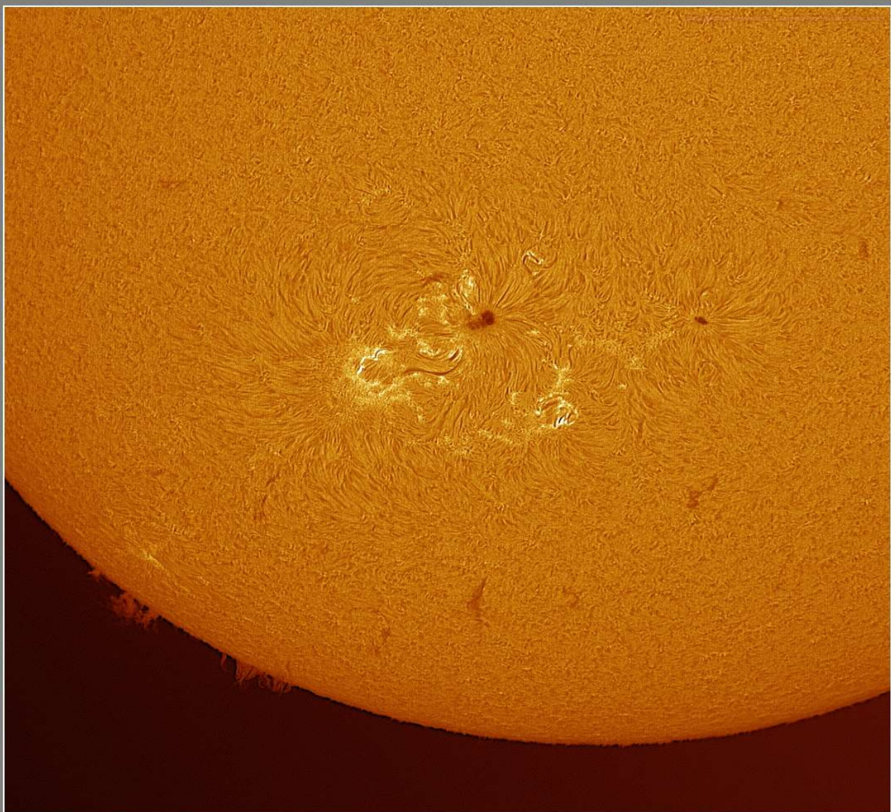
28 Nov 2020, ~10:45h UT. Active regions 12785 & 12786, and prominences. Lunt LS80THa DSII, BF1200, ZWO ASI290MM. Firecapture, Autostakkert, Registax, Photoshop. Transparency good, seeing fair. © Geert Vandenbulcke, Koksijde, Belgium.
